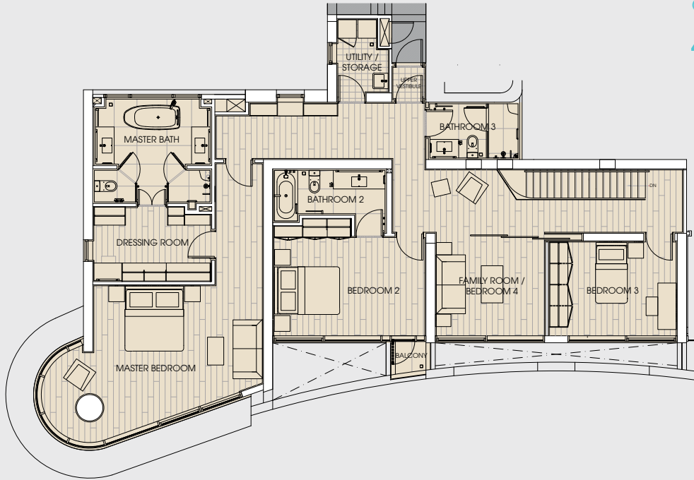
UPPER LEVEL
